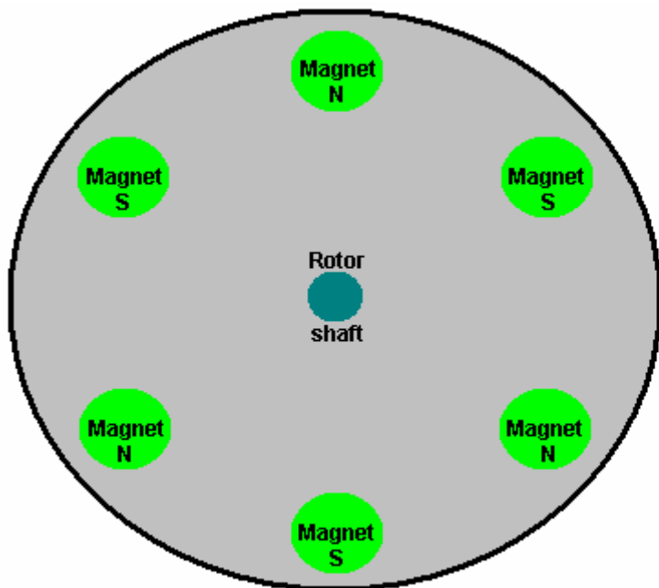
Rotor (1 required)
